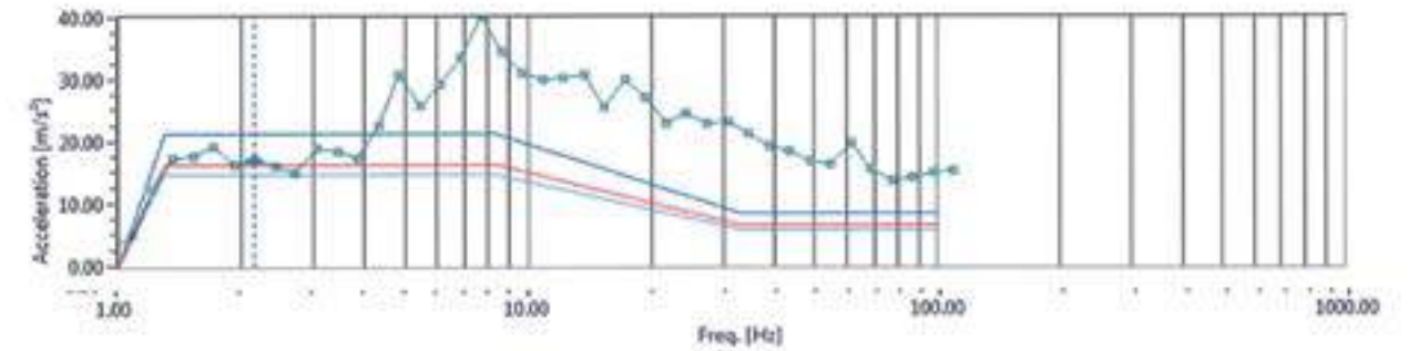
Figure 16 – Seismic Test Result – 800mm Tubeaxial Fan – Z-Direction – Response Spectra
