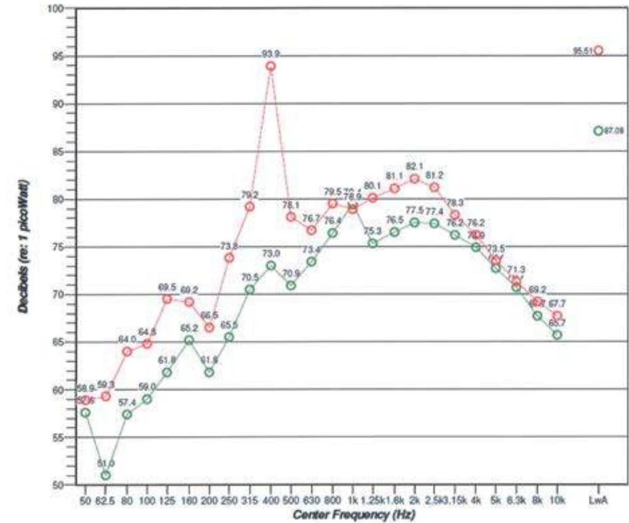
Figure 5 – A-Weighted Outlet Sound Power Level Results – 400mm Jet Fan
