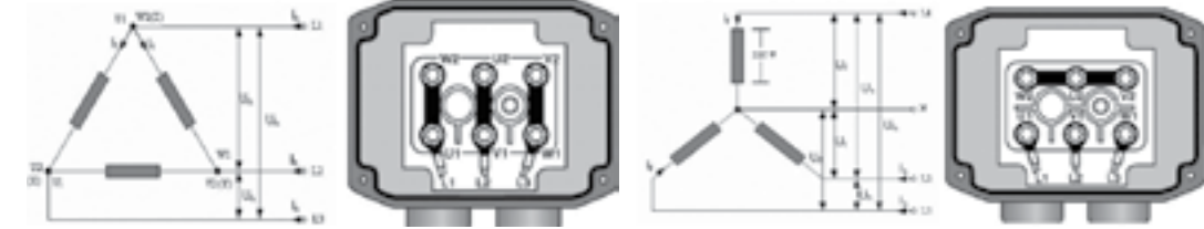
Delta connection
