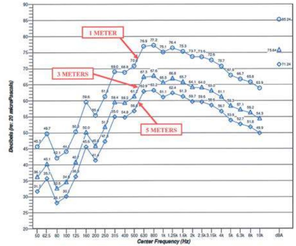
Figure 3 – A-Weighted Outlet Sound Pressure Level Results at 1, 3 and 5 meters – 800mm Tubeaxial
