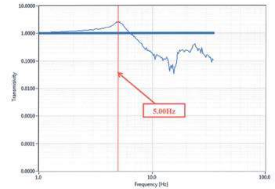
Figure 10 – Natural Frequency Search – 800mm Tubeaxial Fan – Y-Direction
