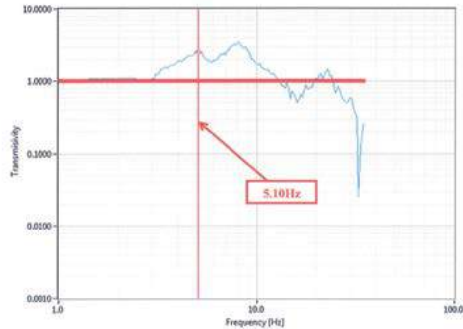
Figure 11 – Natural Frequency Search – 800mm Tubeaxial Fan – Z-Direction
