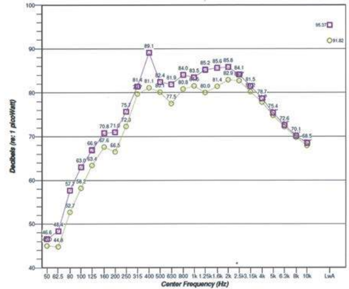
Figure 7 – A-Weighted Total Sound Power Level Results – 400mm Jet Fan
