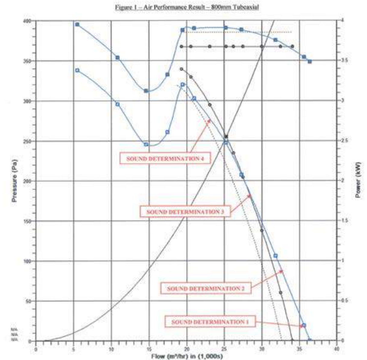
Figure 1 Legend Black Circles – Cvsair Catalog Data (Submittal) Black System Curve (Parabola) – Design Performance Black Dashed Line – AMCA 211 tolerance (applied to Cvsair catalog data) Blue Squares – TCF test data of Cvsair fan (air over motor first)
